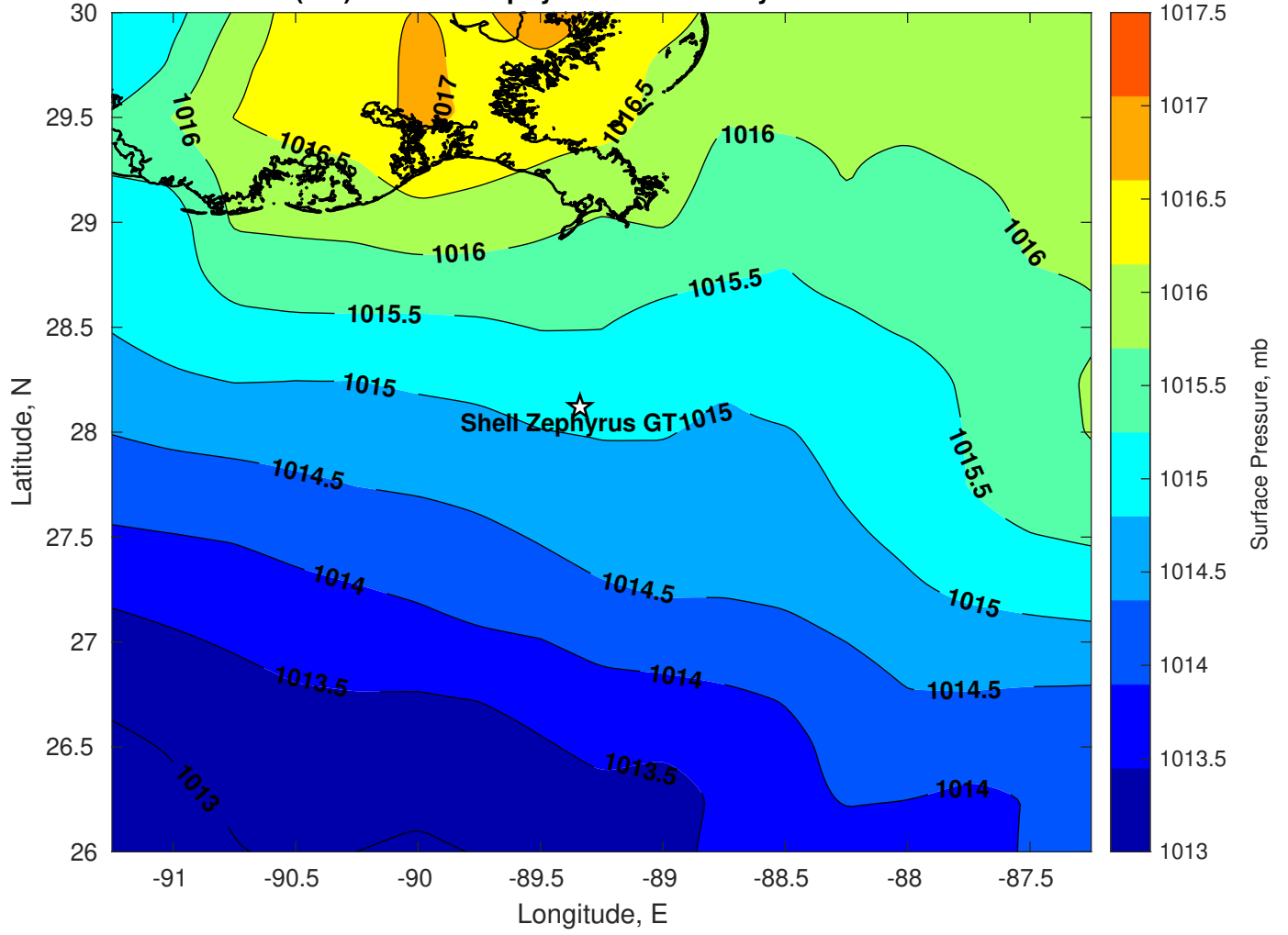
Surface Pressure (mb) for Shell Zephyrus GT at 03-May-2024 18:00:00
