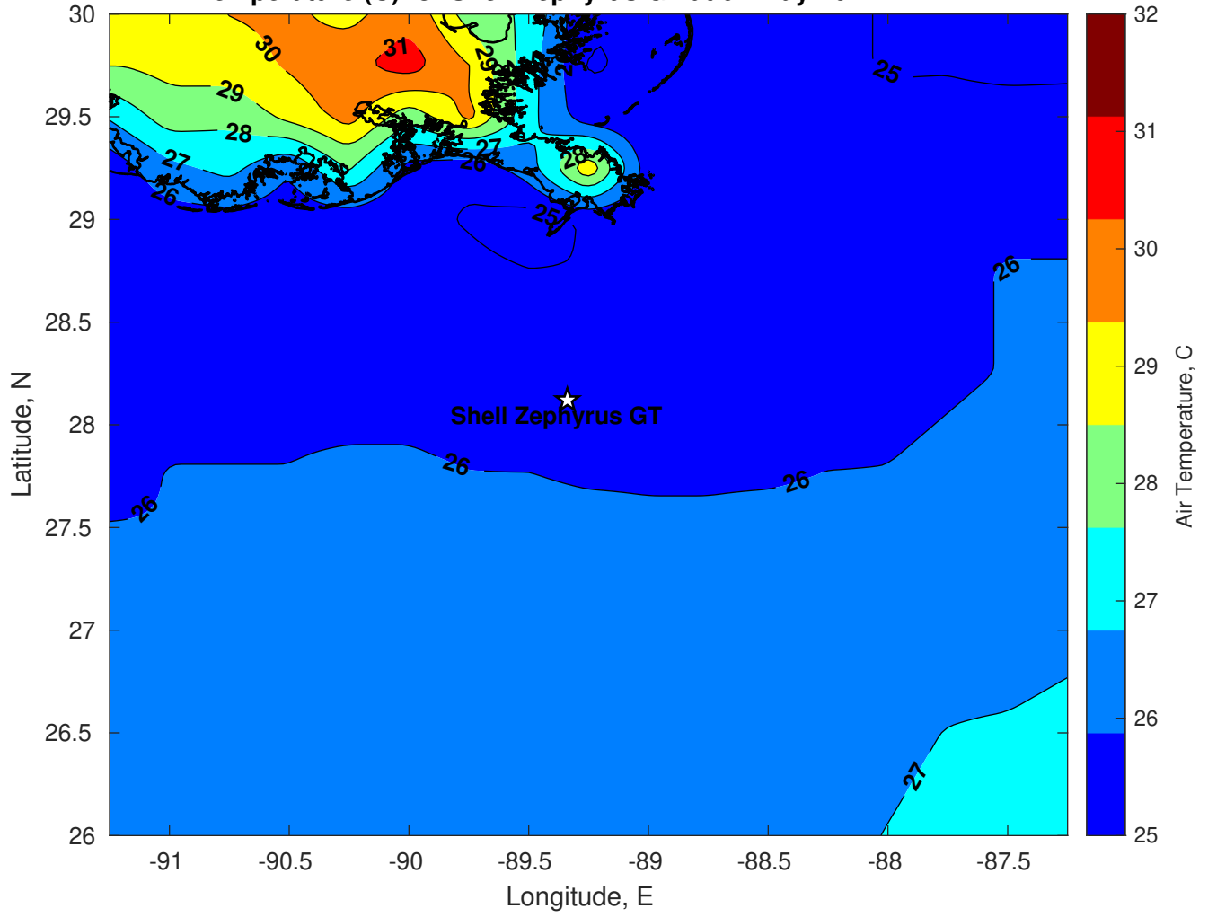
Air Temperature (C) for Shell Zephyrus GT at 02-May-2024
