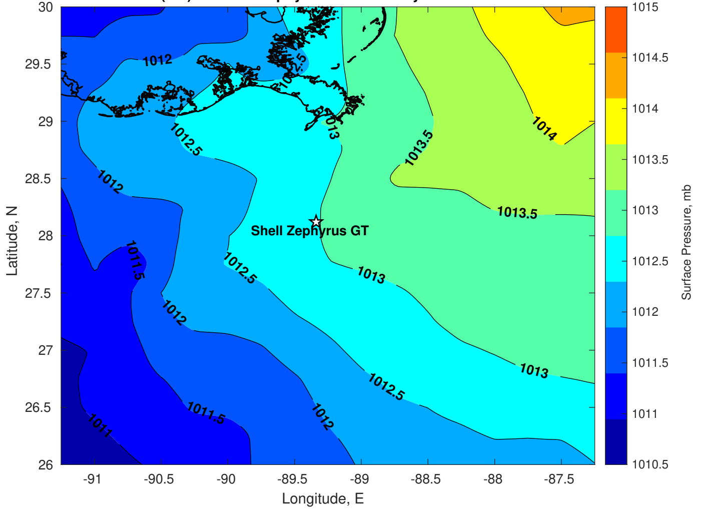
Surface Pressure (mb) for Shell Zephyrus GT at 02-May-2024 18:00:00
