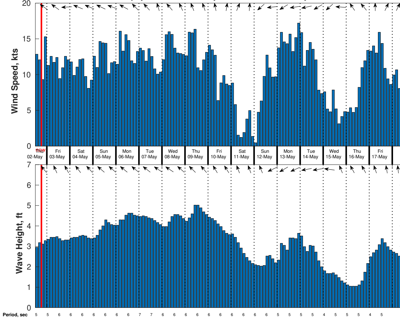
Wind & Wave Forecast for Shell Zephyrus GT from 02-May-2024 12:00:00 to 18-May-2024 12:00:00
