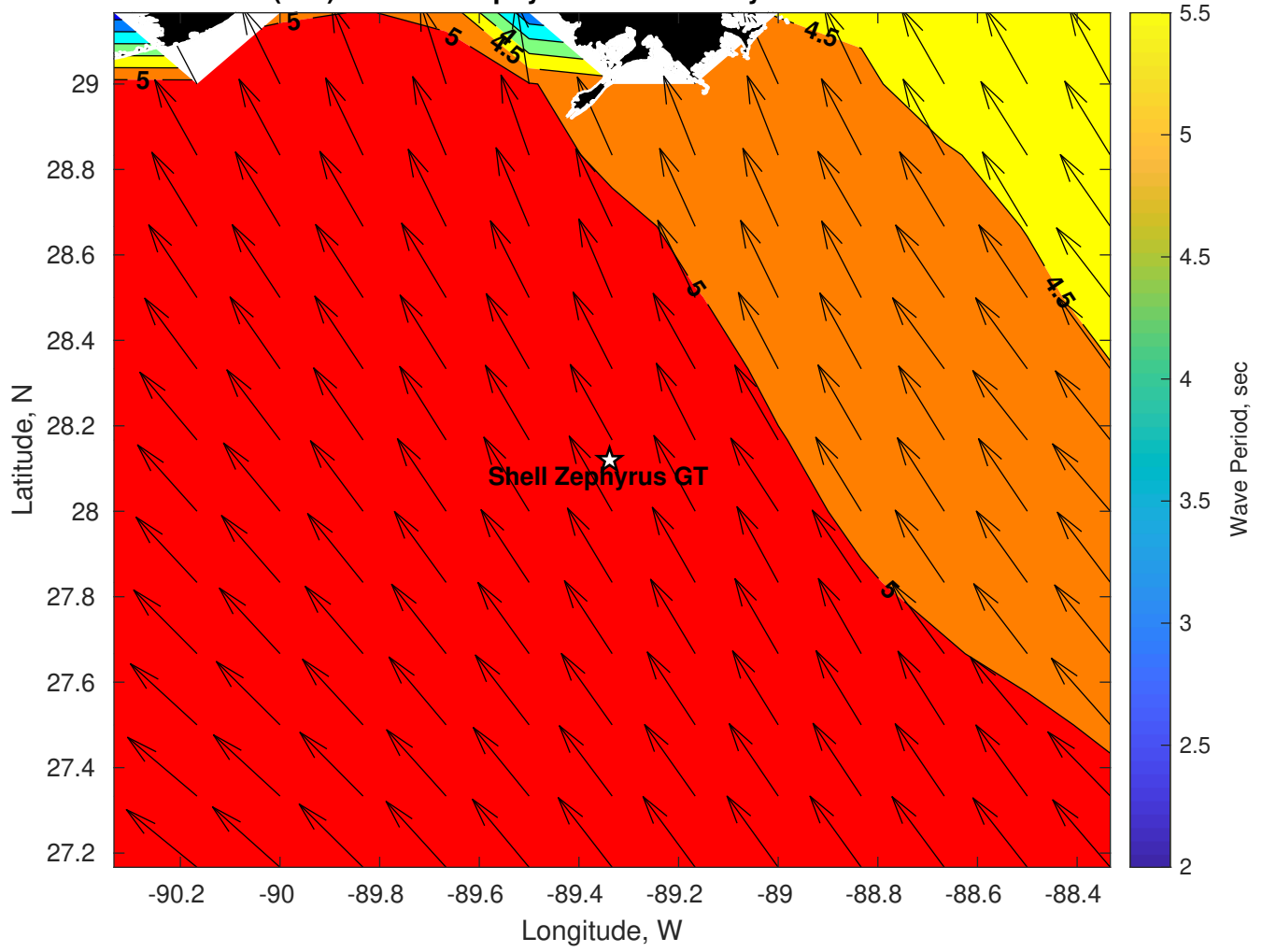
Wave Period (sec) for Shell Zephyrus GT at 03-May-2024 00:00:00
