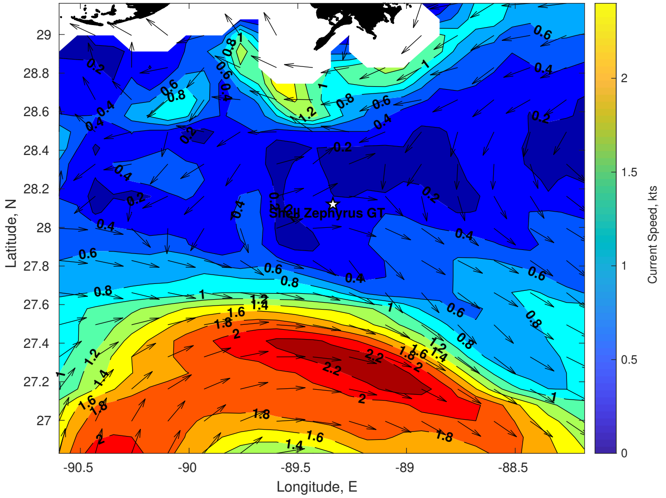
Surface Currents for Shell Zephyrus GT at 02-May-2024 00:00:00
