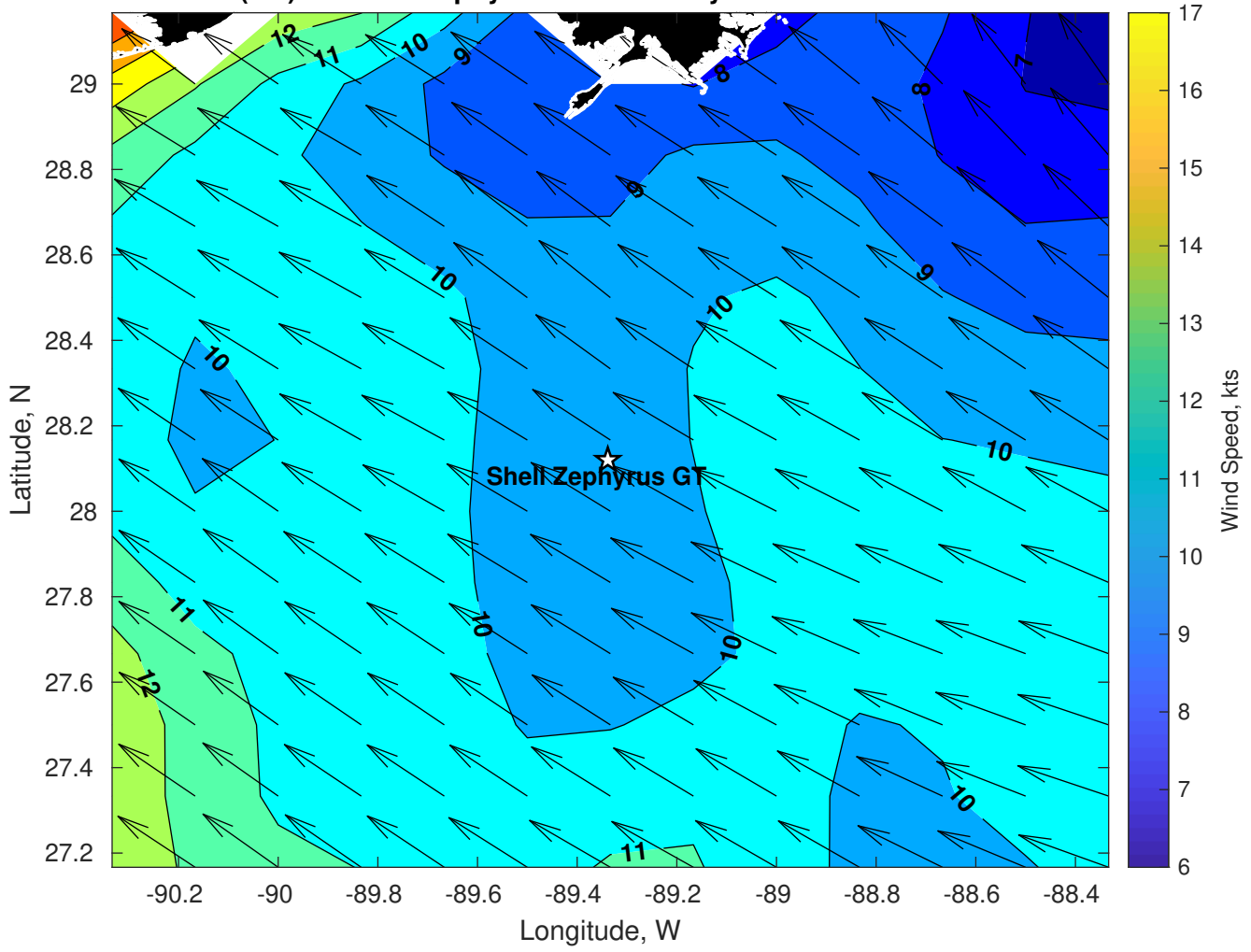
Winds (kts) for Shell Zephyrus GT at 03-May-2024 00:00:00
