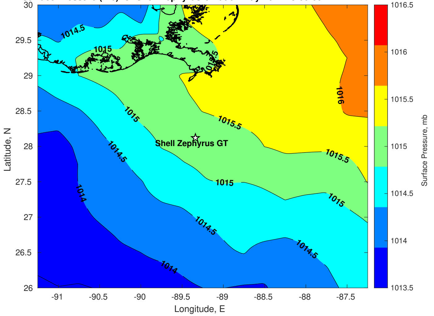
Surface Pressure (mb) for Shell Zephyrus GT at 04-May-2024 18:00:00
