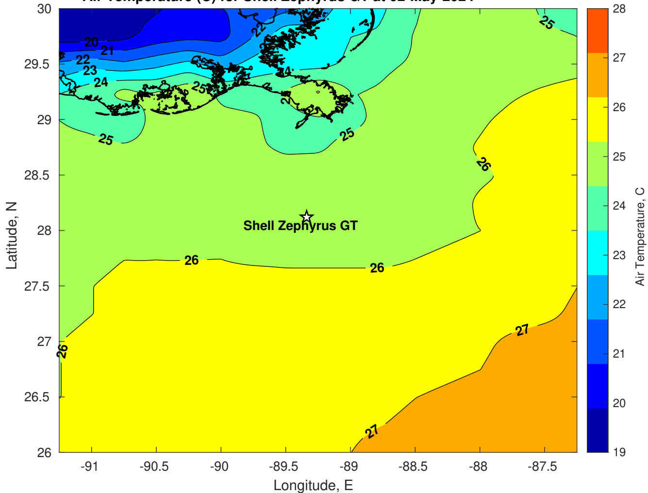
Air Temperature (C) for Shell Zephyrus GT at 02-May-2024
