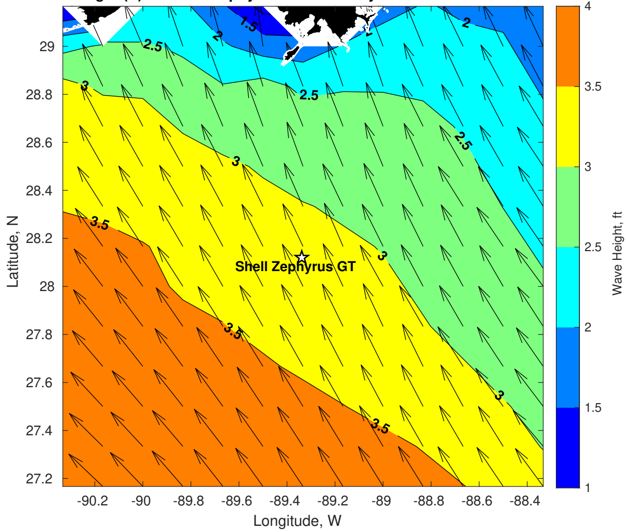
Wave Height (ft) for Shell Zephyrus GT at 03-May-2024 00:00:00
